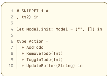
Fig. 12. A confounding snippet commonly retrieved by vector retrieval
